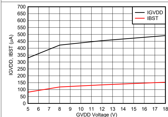
图 6-6. Quiescent Currents vs Supply Voltage
