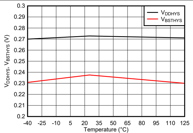
图 6-13. GVDD and BST UVLO Hysteresis vs Temperature
