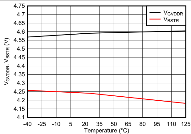
图 6-12. GVDD and BST UVLO Thresholds vs Temperature
