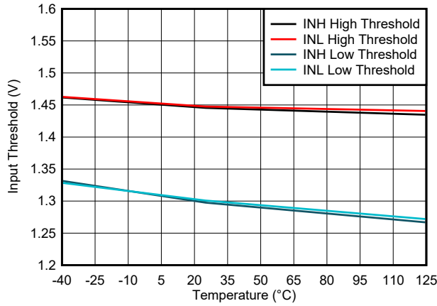
图 6-14. Input Voltage Thresholds vs Temperature
