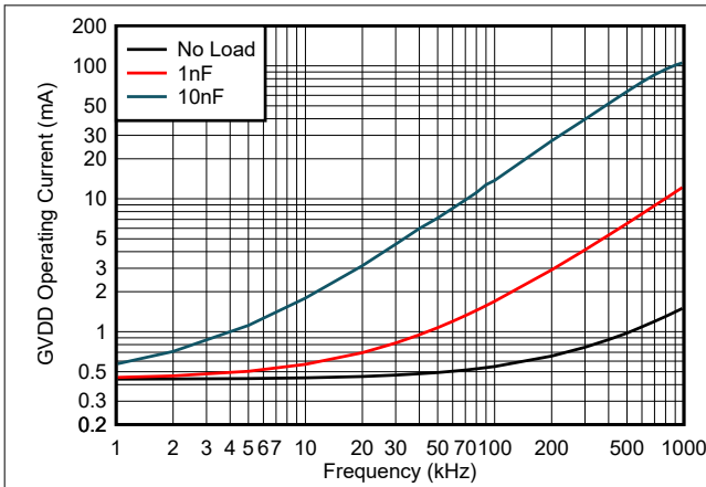
图 6-2. GVDD Operating Current vs Frequency
