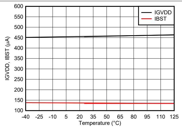
图 6-5. Quiescent Currents vs Temperature
