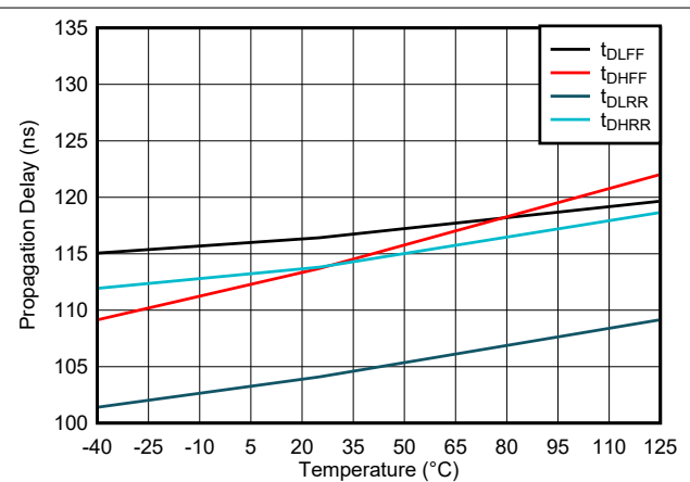
图 6-7. Propagation Delays vs Temperature
