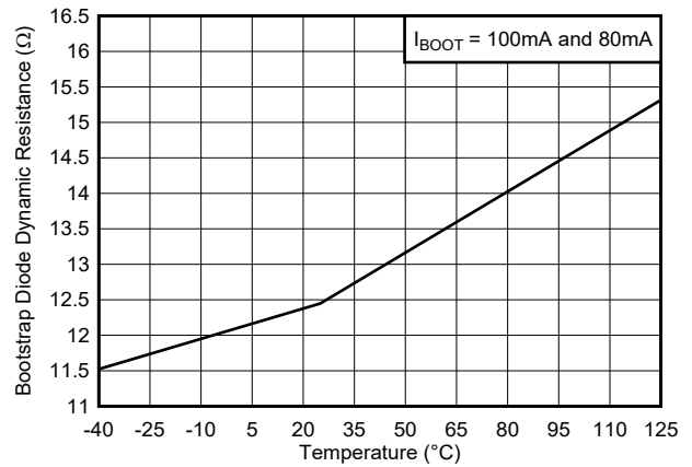
图 6-17. Bootstrap Diode Dynamic Resistance
