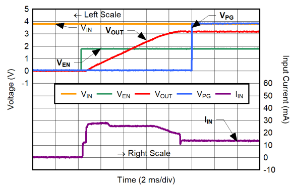
图 6-30. Inrush Current for C_{NR/SS} = 4.7\text{ }\mu\text{F}
