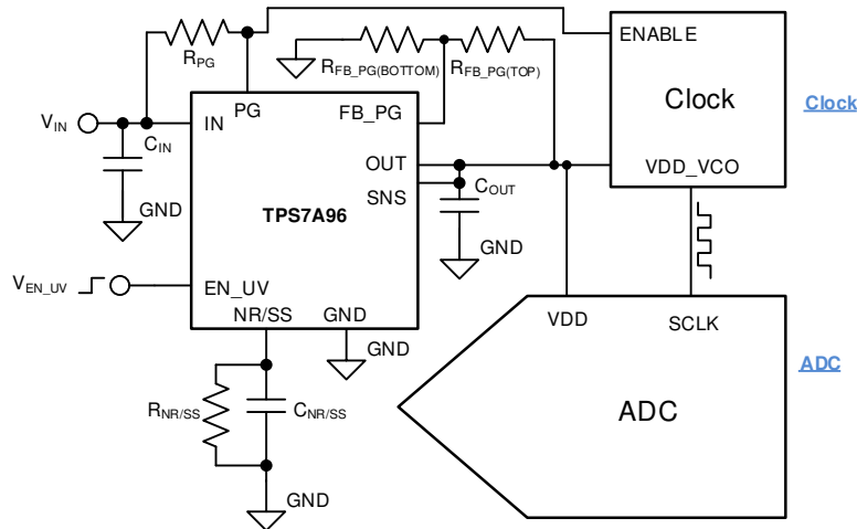
图 8-15. Typical Circuit
