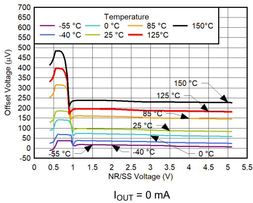
图 6-39. V_{OS} vs V_{NR/SS} and Temperature for I_{OUT} = 0\text{ mA}
