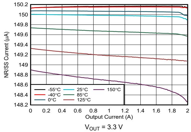
图 6-40. I_{NR/SS} vs I_{OUT} and Temperature for V_{IN} = 3.8\text{ V}
