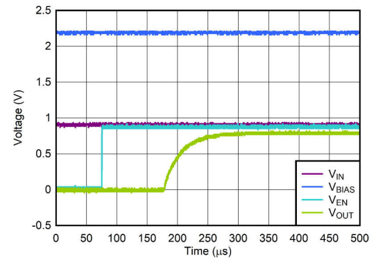
图 6-16. Start-Up With V_{\text{IN}} and V_{\text{BIAS}} Before V_{\text{EN}}
