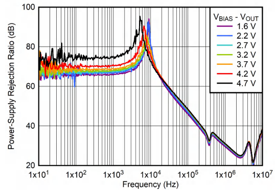
图 6-26. PSRR vs Frequency and V_{BIAS} - V_{OUT}
