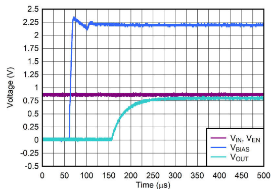
图 6-17. Start-Up With V_{\text{IN}} and V_{\text{EN}} Before V_{\text{BIAS}}
