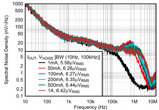
图 6-28. Output Noise vs Frequency and I_{OUT}
