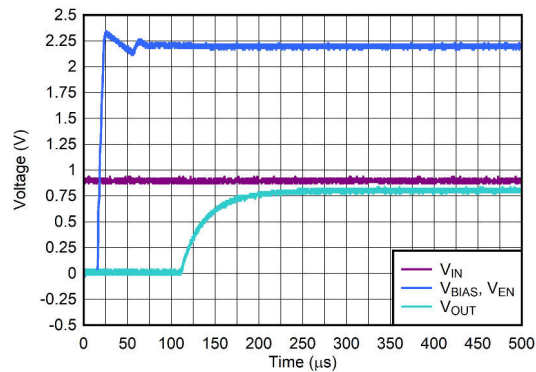
图 6-15. Start-Up With V_{\text{IN}} Before V_{\text{BIAS}} and V_{\text{EN}}
