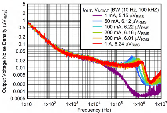
图 6-27. Output Noise vs Frequency and I_{OUT}
