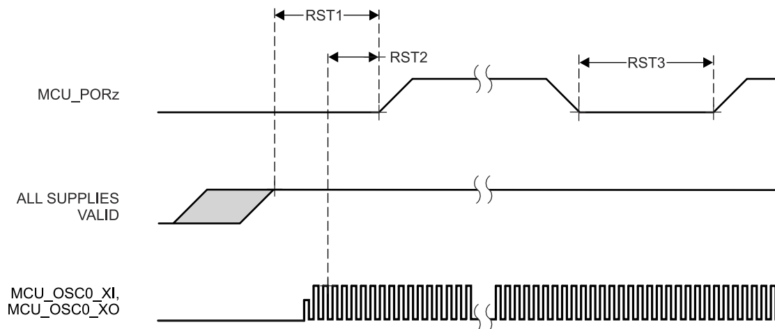
图 7-7. MCU_PORz Timing Requirements
