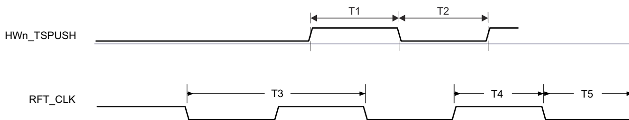
图 7-77. CPTS Timing Requirements
