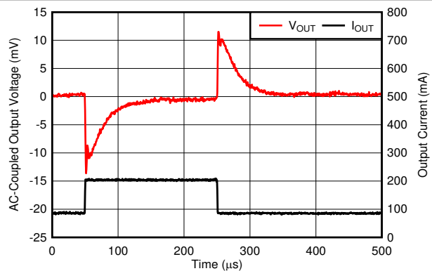
V_{\text{OUT}} = 3.3\text{ V} , I_{\text{OUT}} = 90\text{ mA to } 200\text{ mA} , I_{\text{OUT}} slew rate = 1\text{ A}/\mu\text{s} , T_J = 150^\circ\text{C}
