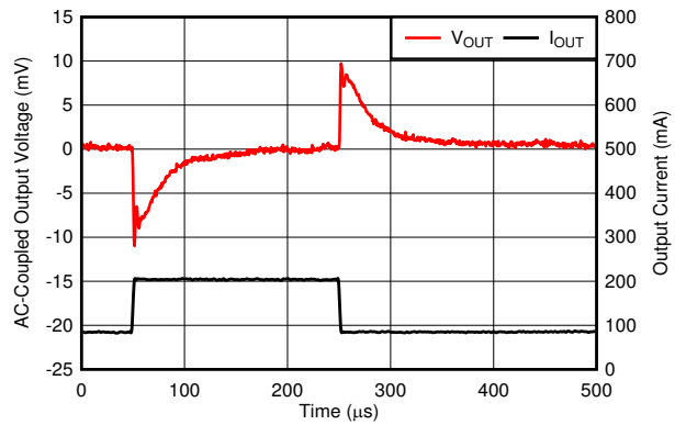
V_{\text{OUT}} = 3.3\text{ V} , I_{\text{OUT}} = 90\text{ mA to } 200\text{ mA} , I_{\text{OUT}} slew rate = 1\text{ A}/\mu\text{s} , T_J = 25^\circ\text{C}
