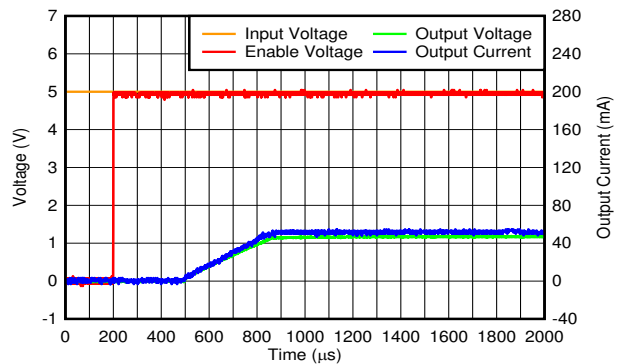
图 6-76. Start-Up Inrush Current With C_{OUT} = 1\ \mu\text{F}
