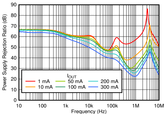
V_{\text{IN}} = 1.65\text{ V} , C_{\text{IN}} = 0\ \mu\text{F} , V_{\text{OUT}} = 0.65\text{ V}
