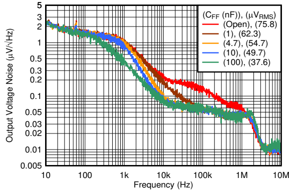
图 6-73. Output Noise vs Frequency and C_{FF}
