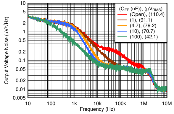
图 6-74. Output Noise vs Frequency and C_{FF}
