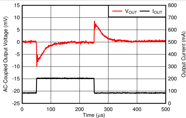
V_{\text{OUT}} = 3.3\text{ V} , I_{\text{OUT}} = 90\text{ mA to } 200\text{ mA} , I_{\text{OUT}} slew rate = 1\text{ A}/\mu\text{s} , T_J = -40^\circ\text{C}
