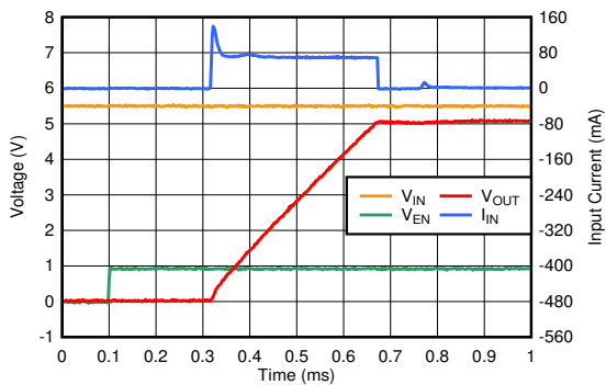
图 6-75. Start-Up Inrush Current With C_{OUT} = 1\ \mu\text{F}
