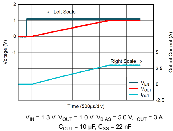
图 6-15. Start-Up Waveform for C_{SS} = 22\text{ nF}
