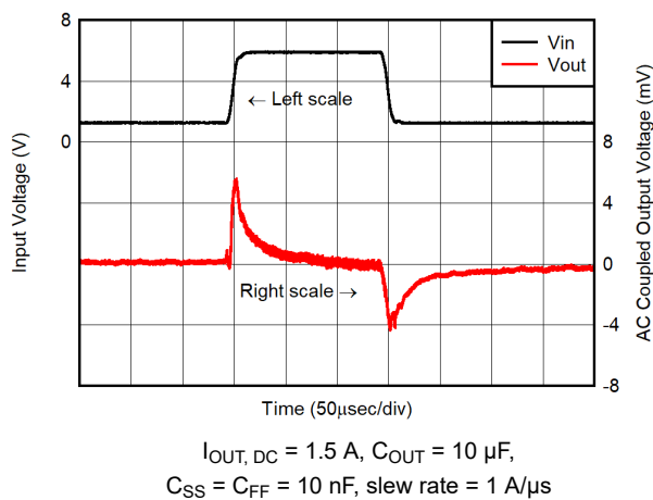
图 6-17. Line Transient for V_{OUT} With Bias
