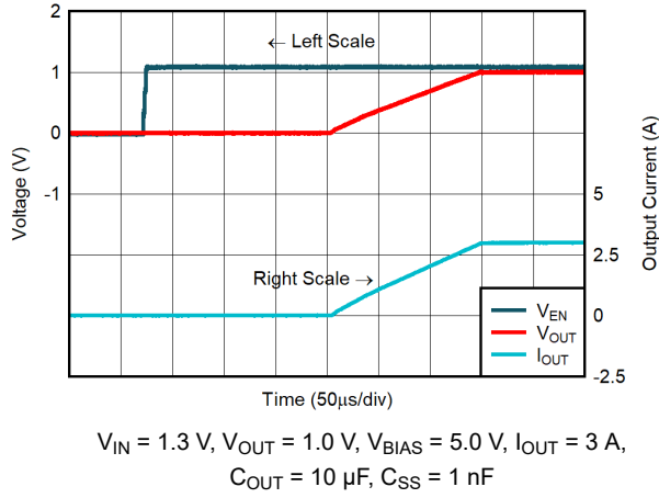
图 6-13. Start-Up Waveform for C_{SS} = 1\text{ nF}
