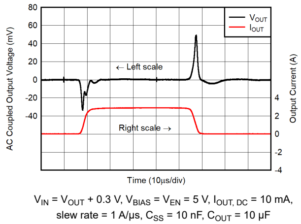
图 6-16. Load Transient for V_{OUT} With Bias
