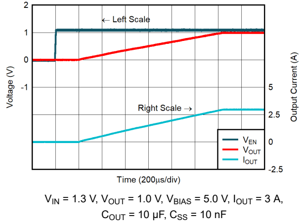
图 6-14. Start-Up Waveform vs Time for C_{SS} = 10\text{ nF}
