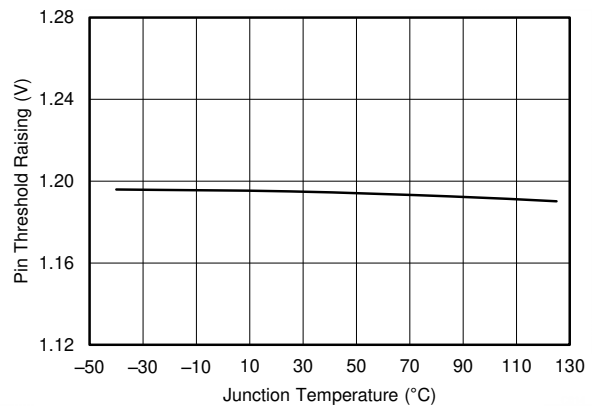
图 6-18. EN Pin Threshold Rising vs Temperature
