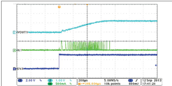
图 8-3. PSM Mode Buck1, Soft-Start with No Load
