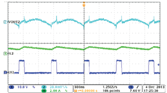
图 8-12. Buck2, Steady State Operation with Full Load
