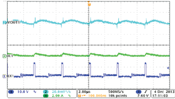
图 8-9. PSM Mode Buck1, Steady State Operation with Light Load
