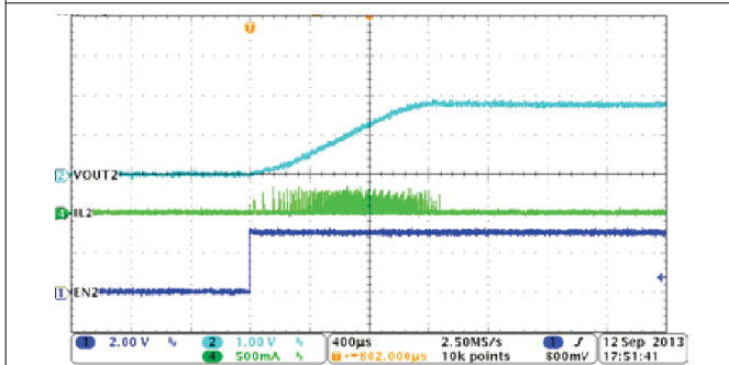
图 8-5. PSM Mode Buck2, Soft-Start with No Load
