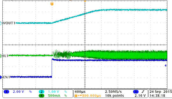
图 8-27. PWM Mode, Buck1, Soft-Start with No Load
