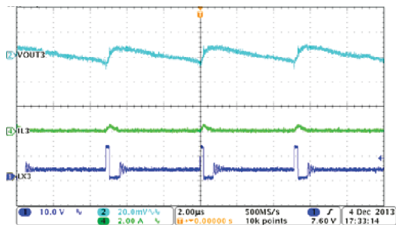
图 8-13. PSM Mode Buck3, Steady State Operation with Light Load
