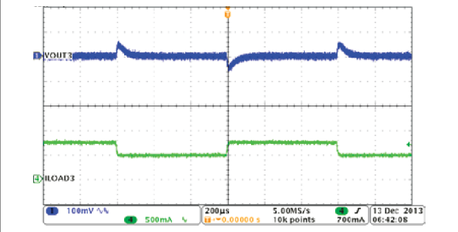
图 8-20. Buck3, Load Transient, 0.5 to 0.75 A SR = 0.25A/µs
