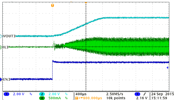
图 8-31. PWM Mode, Buck3, Soft-Start with No Load
