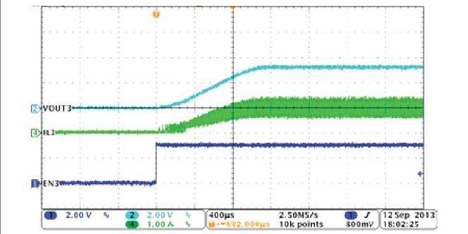
图 8-8. PSM Mode Buck3, Soft-Start with Full Load
