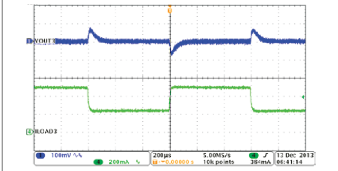
图 8-19. Buck3, Load Transient, 0.25 to 0.5 A SR = 0.25 A/µs
