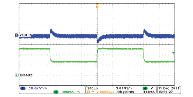
图 8-17. Buck2, Load Transient, 0.25 to 0.5 A SR = 0.25 A/µs
