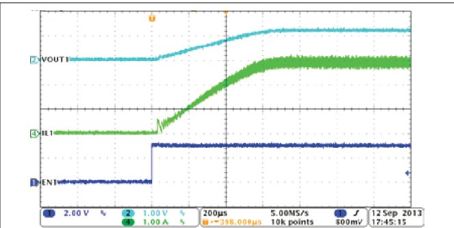
图 8-4. PSM Mode Buck1, Soft-Start With Full Load
