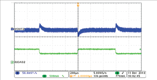
图 8-18. Buck2, Load Transient, 0.5 to 0.75 A SR = 0.25A/µs
