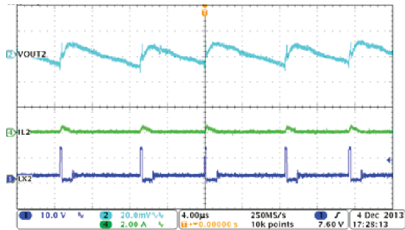
图 8-11. PSM Mode Buck2, Steady State Operation With Light Load
