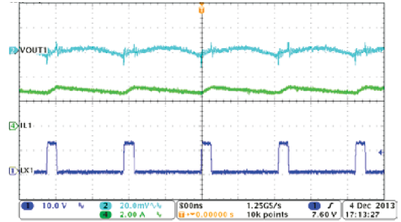
图 8-10. Buck1, Steady State Operation with Full Load
