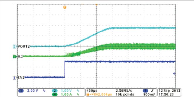
图 8-6. PSM Mode Buck2, Soft-Start with Full Load
