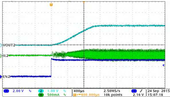
图 8-29. PWM Mode, Buck2, Soft-Start with No Load
