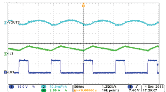
图 8-14. Buck3, Steady State Operation with Full Load
