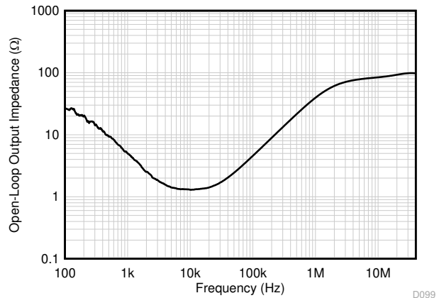
图 6-30. Open-Loop Output Impedance vs Frequency
