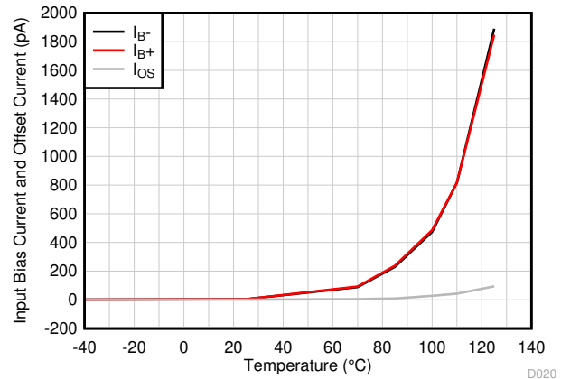
图 6-14. Input Bias Current and Offset Current vs Temperature
