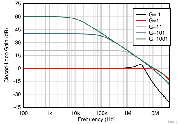
图 6-12. Closed-Loop Gain vs Frequency
