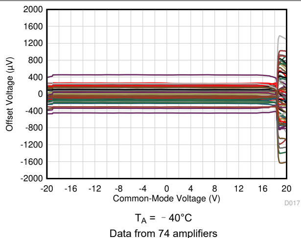
图 6-9. Offset Voltage vs Common-Mode Voltage
