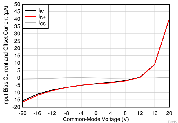
图 6-13. Input Bias Current and Offset Current vs Common-Mode Voltage
