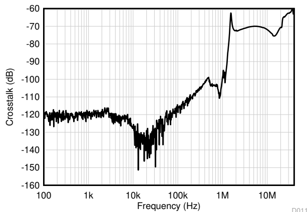
图 6-42. Channel Separation vs Frequency
