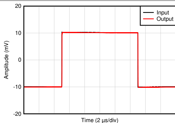
图 6-35. Positive Overload Recovery
