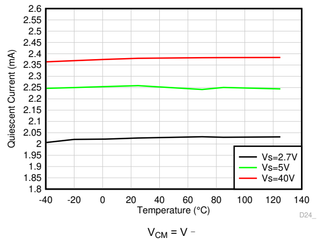
图 6-28. Quiescent Current vs Temperature
