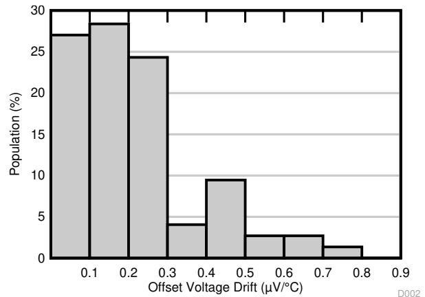
Distribution from 74 amplifiers 图 6-2. Offset Voltage Drift Distribution
