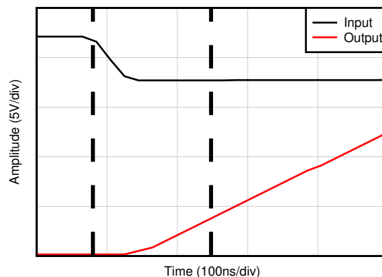
图 6-36. Negative Overload Recovery
