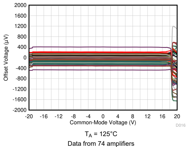
图 6-7. Offset Voltage vs Common-Mode Voltage
