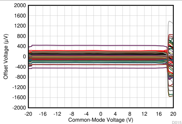
T_A = 25^\circ\text{C} Data from 74 amplifiers 图 6-5. Offset Voltage vs Common-Mode Voltage
