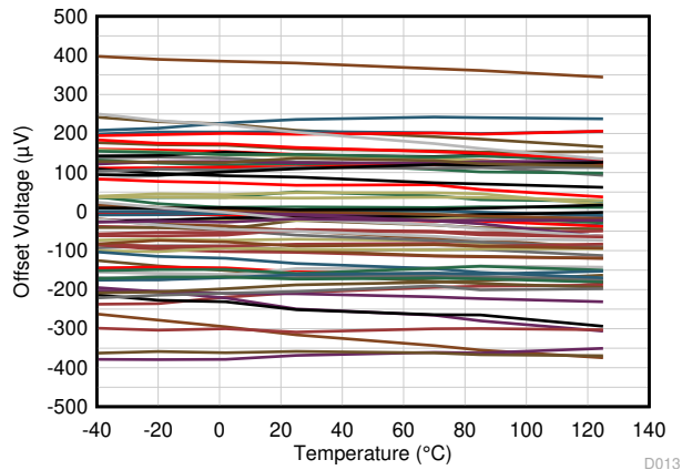
V_{CM} = V^- Data from 74 amplifiers 图 6-3. Offset Voltage vs Temperature
