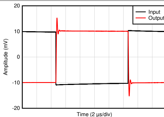
图 6-36. Negative Overload Recovery
