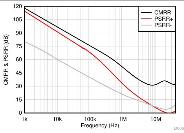
图 6-20. CMRR and PSRR vs Frequency
