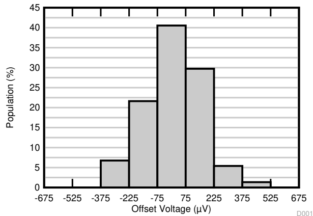
Distribution from 74 amplifiers, T_A = 25^\circ\text{C} 图 6-1. Offset Voltage Production Distribution
