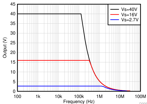
图 6-41. Maximum Output Voltage vs Frequency
