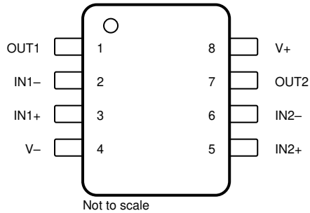
图 5-3. OPA2992-Q1 D and DGK Package, 8-Pin SOIC and VSSOP (Top View)
