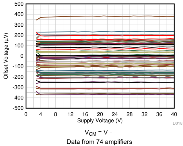
图 6-11. Offset Voltage vs Power Supply
