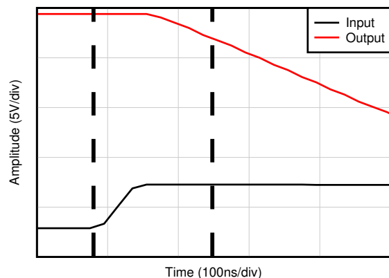
图 6-35. Positive Overload Recovery
