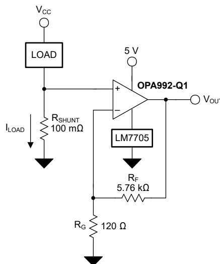
图 8-1. OPAx992-Q1 in a Low-Side, Current-Sensing Application
