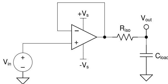
图 7-7. Extending Capacitive Load Drive With the OPA992-Q1
