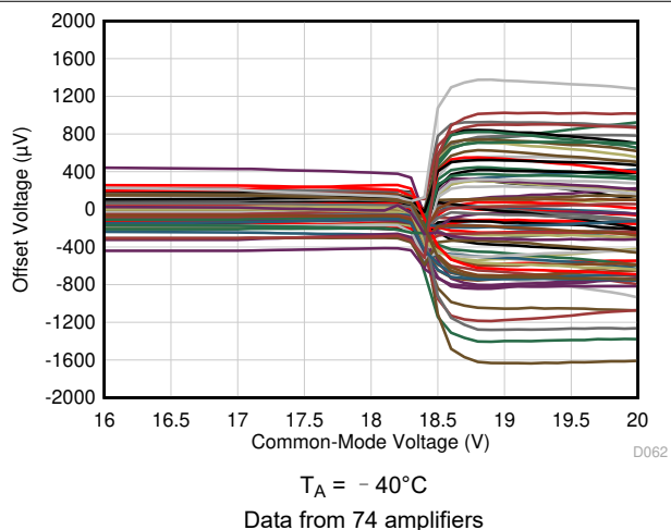
图 6-10. Offset Voltage vs Common-Mode Voltage (Transition Region)
