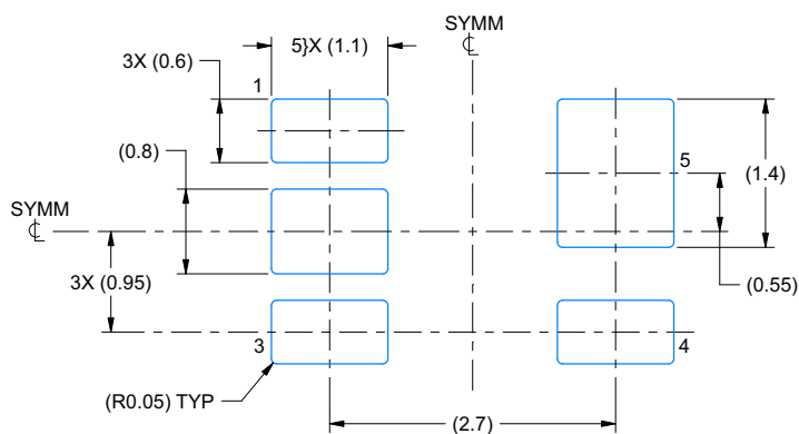
LAND PATTERN EXAMPLE EXPOSED METAL SHOWN SCALE:15X
