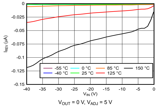
图 6-16. Reverse Current vs. Input Voltage
