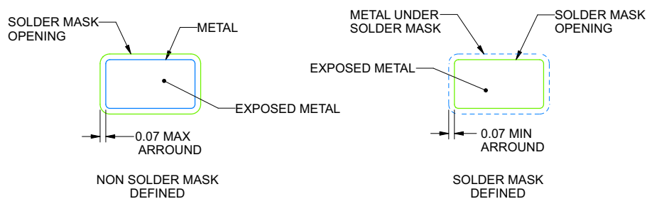
SOLDERMASK DETAILS
