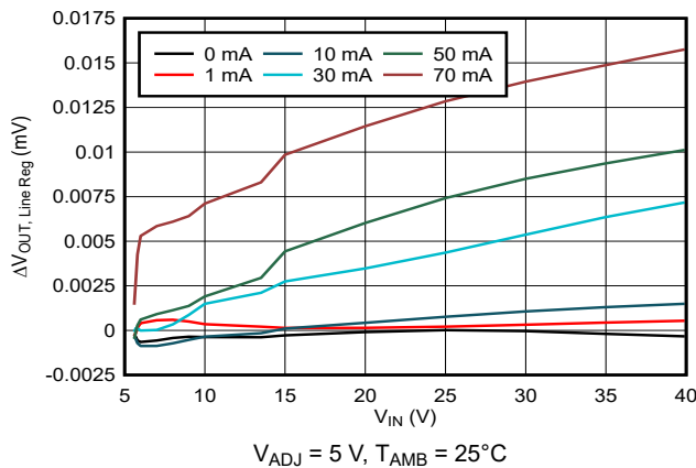
图 6-3. Line Regulation
