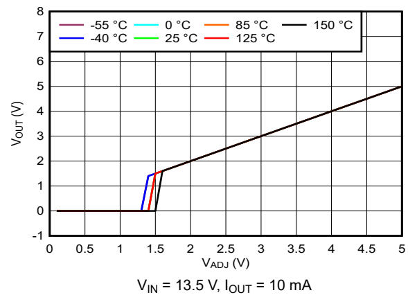
图 6-6. Output Voltage vs Adjustable Reference Voltage
