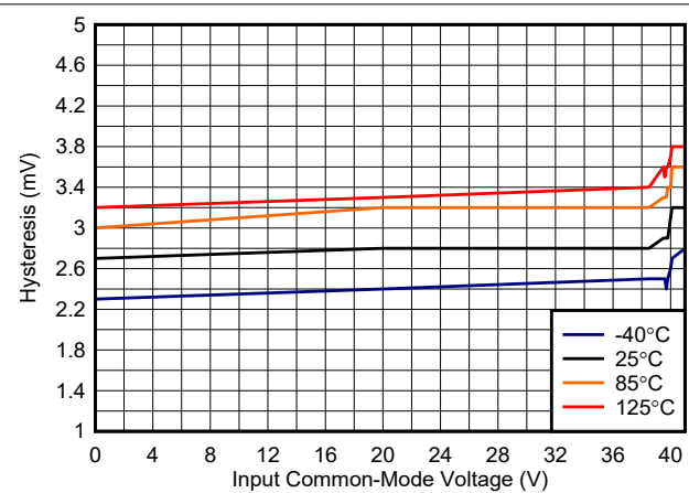
图 6-8. Hysteresis vs. Common-Mode, 40 V
