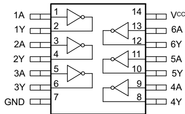
图 5-1. SN54AHCT04 J or W Package, 14-Pin (Top View)
