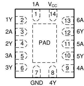
图 5-2. SN74AHCT04 RGY or BQA Package, 14-Pin (Top View)
