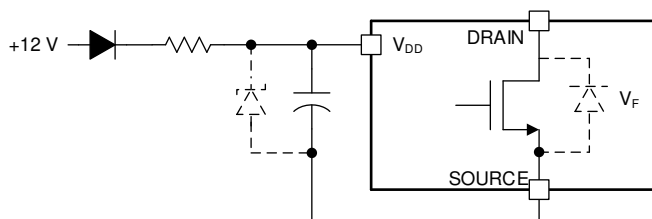
图 9-8. Suggested Bootstrap Regulation Circuit
