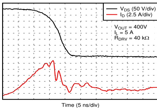
图 9-5. Turn-On Waveform in Application Example
