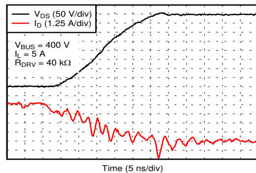
图 9-6. Turn-Off Waveform in Application Example
