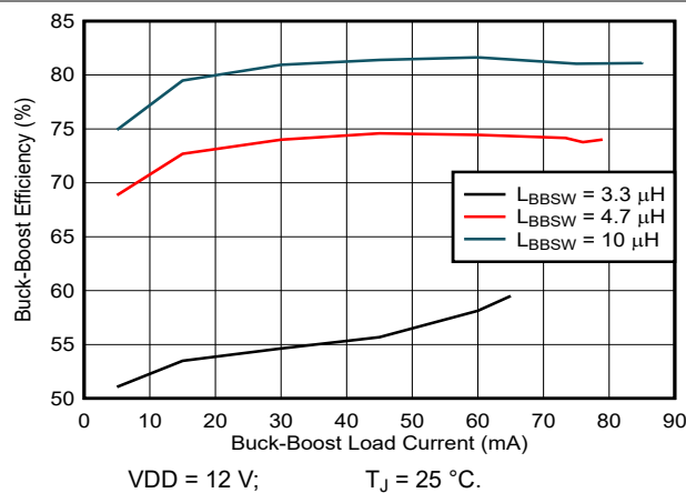
图 9-3. Buck-Boost Efficiency vs Load when I_{BBSW,PK} = I_{BBSW,PK(low)}
