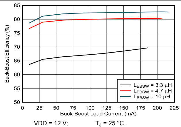
图 9-4. Buck-Boost Efficiency vs Load when I_{BBSW,PK} = I_{BBSW,PK(high)}
