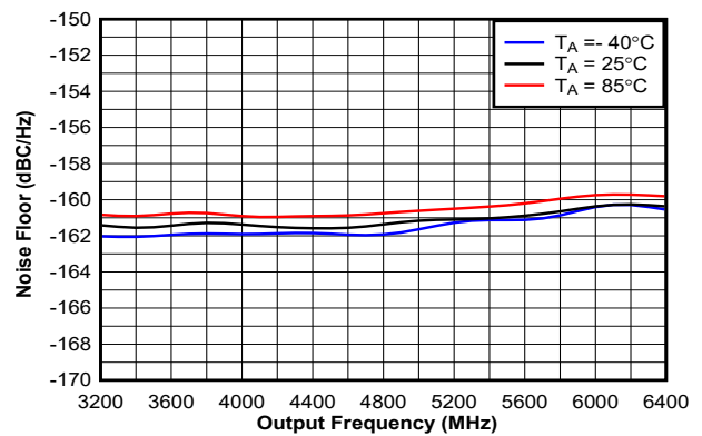
图 6-9. Noise Floor in x2 Multiplier Mode
