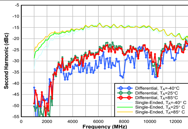
图 6-16. Second Harmonic in Buffer Mode
