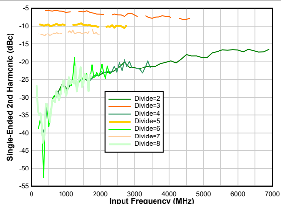
图 6-17. Second Harmonic in Divide Mode (Single-Ended)
