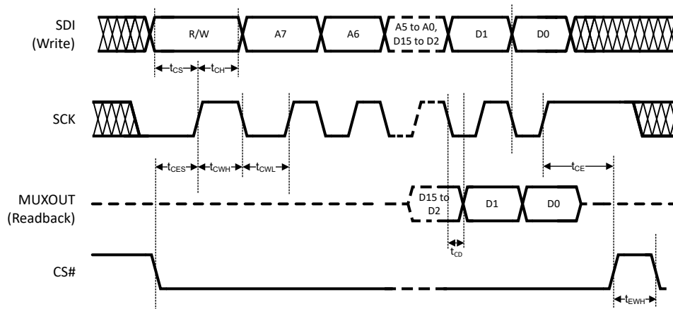
图 6-1. Serial Data Input Timing Diagram
