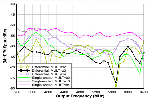
图 6-23. Multiplier Intermodulation (M+1)/M Spur
