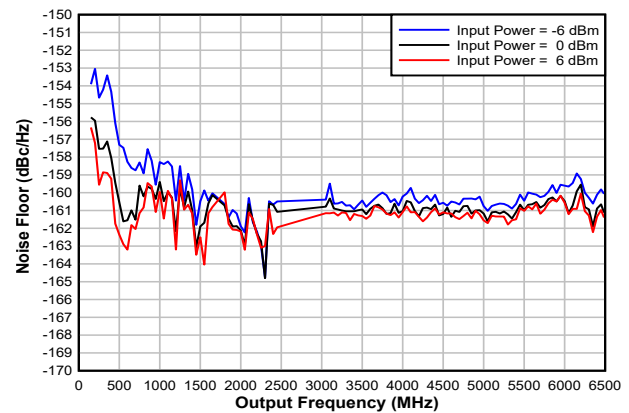
图 6-3. Noise Floor in Buffer Mode
