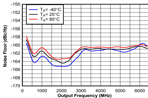
图 6-10. Noise Floor in Divide by 2 Mode
