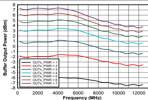
图 6-12. Single-Ended Output Power
