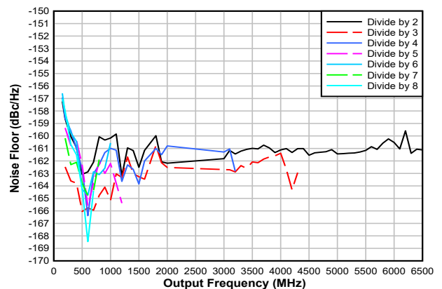
图 6-11. Noise Floor in Divider Mode
