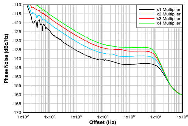
图 6-6. Multiplier Phase Noise Plot at 6 GHz Output
