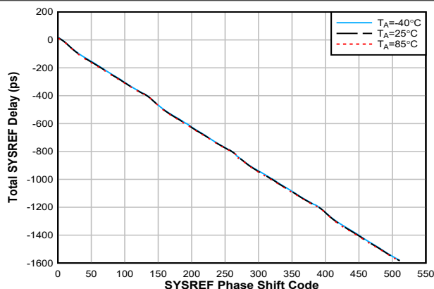
图 6-28. SYSREF Delay vs. Temperature and Code (F out = 10 GHz)
