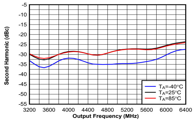
图 6-19. Second Harmonic in Multiply X2 Mode (Differential)
