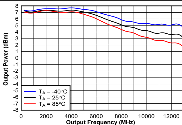
图 6-13. Single-Ended Output Power
