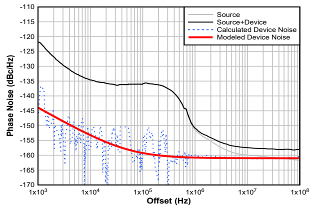
图 6-2. Buffer Phase Noise Plot at 6 GHz Output
