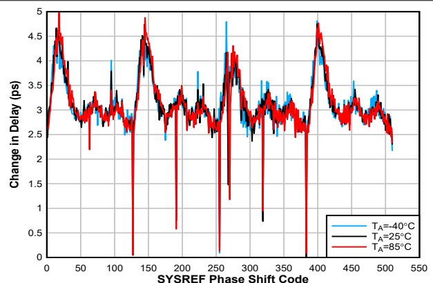
图 6-29. SYSREF Delta Delay vs. Temperature and Code (F out =10 GHz)
