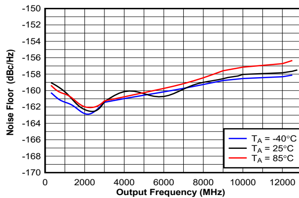
图 6-8. Noise Floor in Buffer Mode
