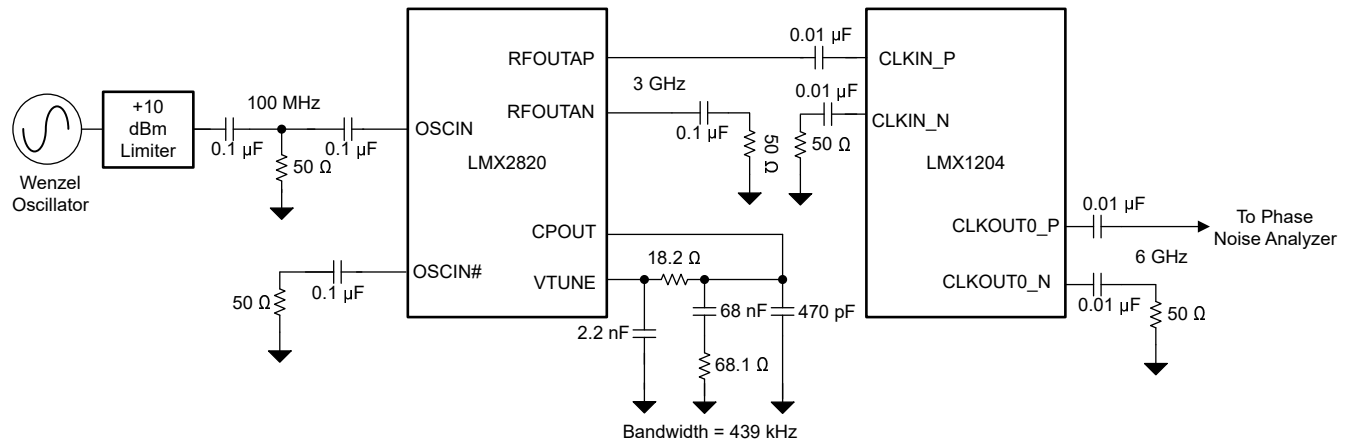
图 8-1. Typical Application Schematic
