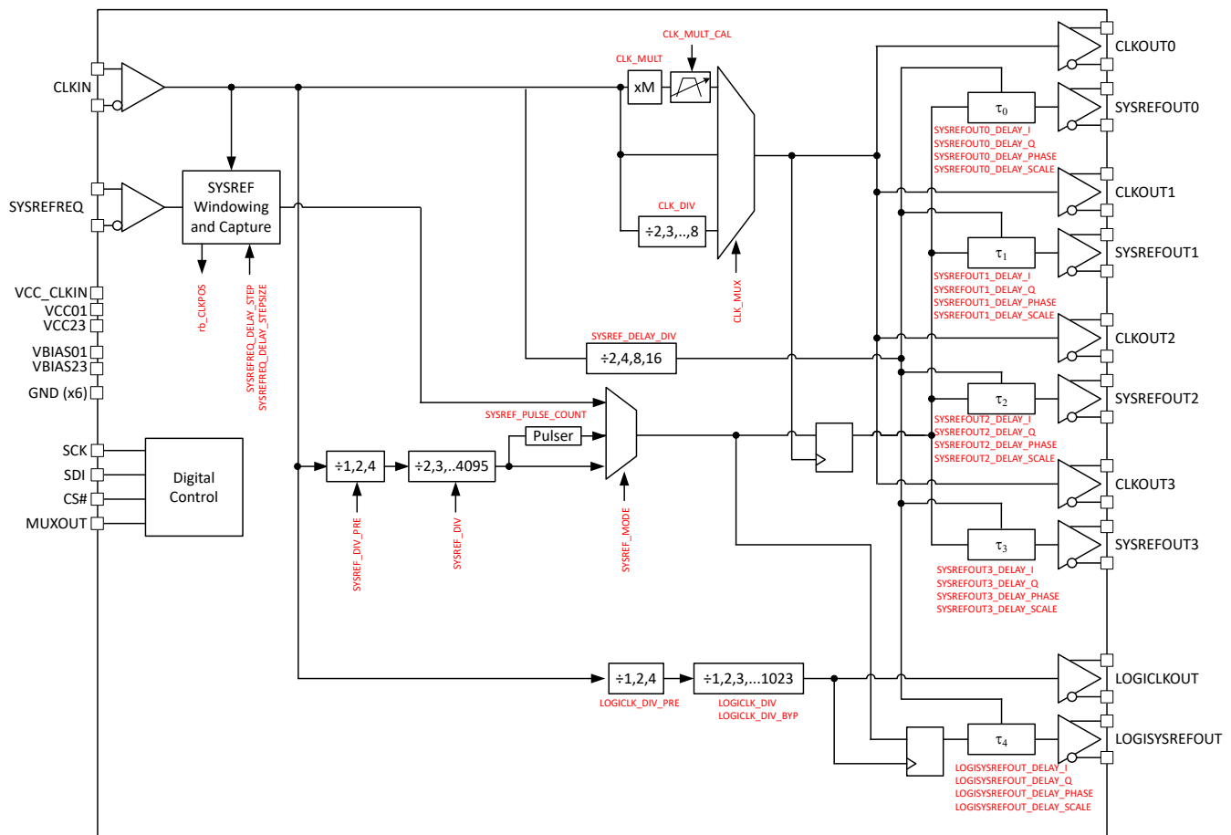
图 7-1. Functional Block Diagram
