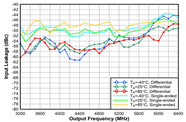
图 6-21. Multiplier 1/2 Sub-Harmonic in X2 Mode
