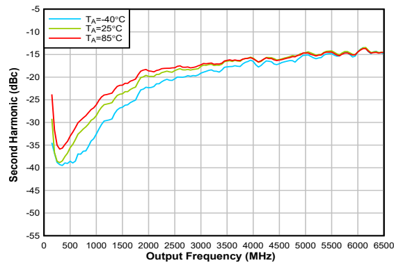
图 6-18. Second Harmonic in Divide by 2 Mode (Single-Ended)
