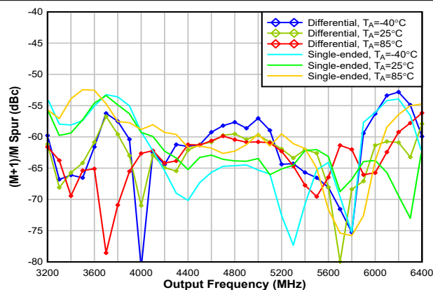
图 6-22. Multiplier Intermodulation Spur (MULT=2)
