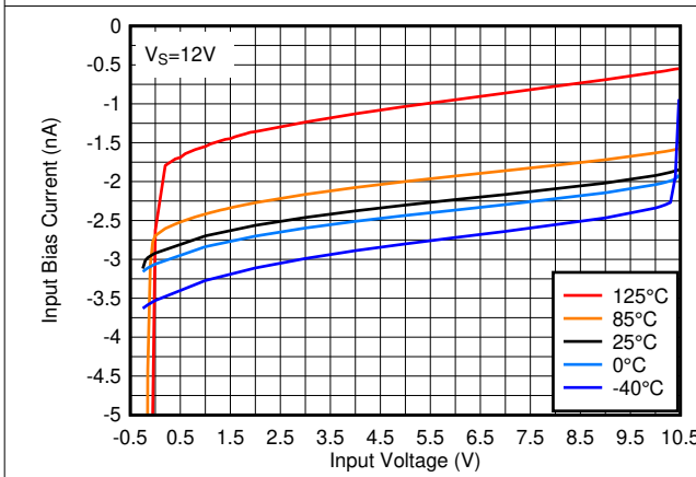
图 3-23. Input Bias Current vs. Input Voltage at 12V
