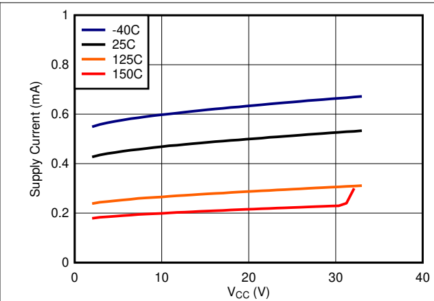
图 3-2. Supply Current vs. Supply Voltage LM2903E-Q1 Only
