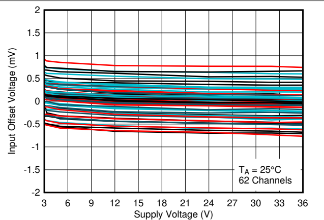
图 3-18. Input Offset Voltage vs. Supply Voltage at 25^\circ\text{C}
