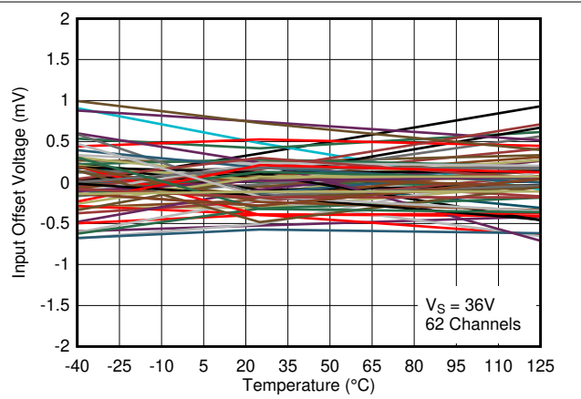
图 3-16. Input Offset Voltage vs. Temperature at 36V
