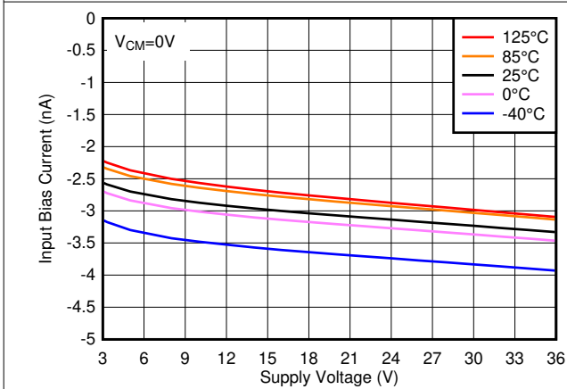
图 3-21. Input Bias Current vs. Supply Voltage
