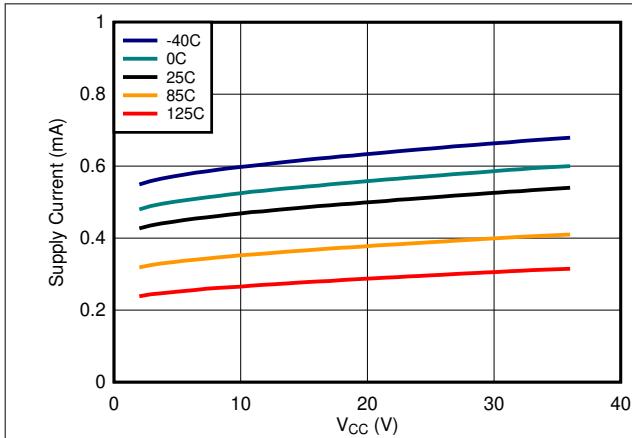
图 3-1. Supply Current vs. Supply Voltage
