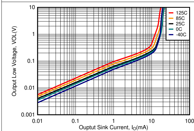
图 3-5. Output Low Voltage vs. Output Current
