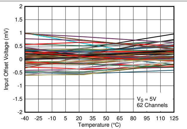
图 3-14. Input Offset Voltage vs. Temperature at 5V
