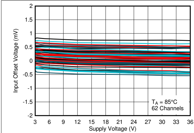
图 3-19. Input Offset Voltage vs. Supply Voltage at 85°C
