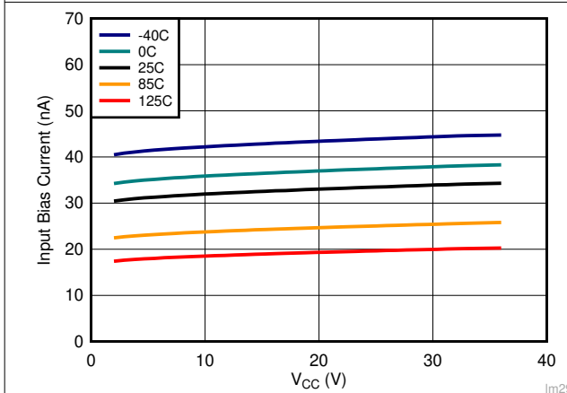
图 3-3. Input Bias Current vs. Supply Voltage
