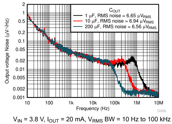
图 6-68. Noise vs Frequency and C_{OUT}
