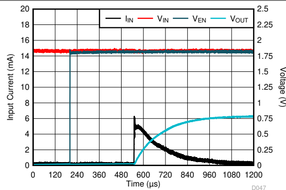
图 6-81. Start-Up
