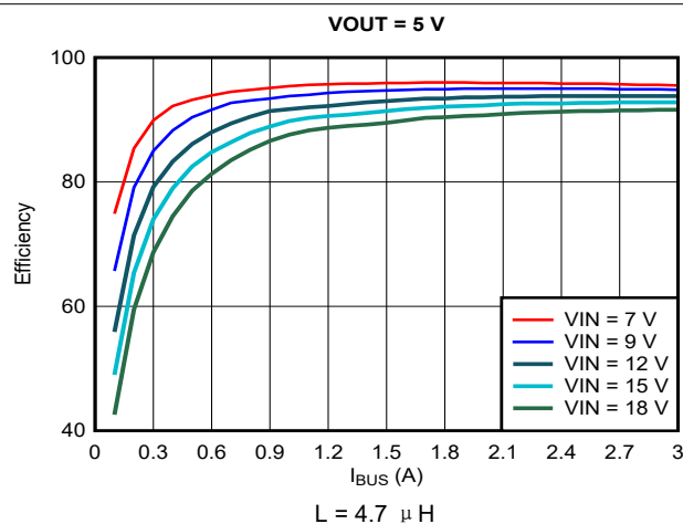
图 10-6. Efficiency vs Output Current ( I_{OUT} ), V_{OUT} = 5\text{ V}
