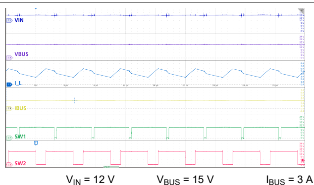
图 10-26. Buck-Boost Mode: Nominal V_{IN} , 3 A Load
