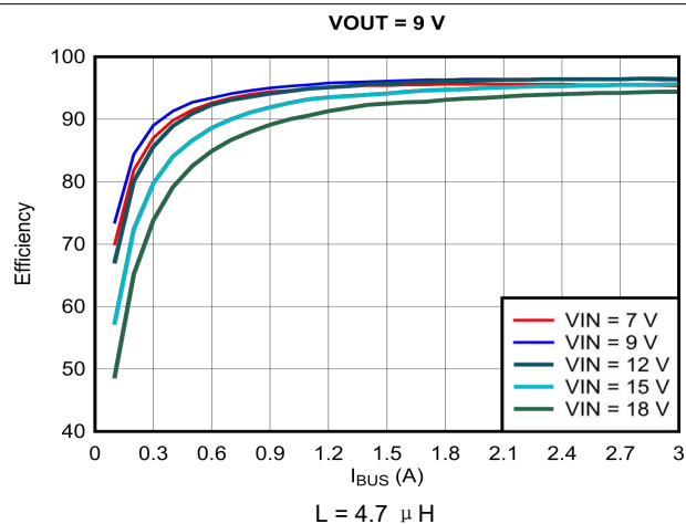
图 10-7. Efficiency vs Output Current ( I_{OUT} ), V_{OUT} = 9\text{ V}
