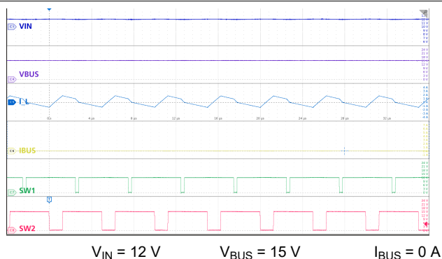
图 10-25. Buck-Boost Mode: Nominal V_{IN} , No Load
