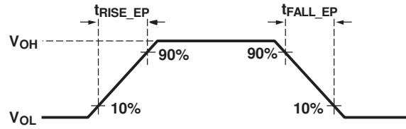
图 8-3. USB Endpoint Transmitter Rise and Fall Time
