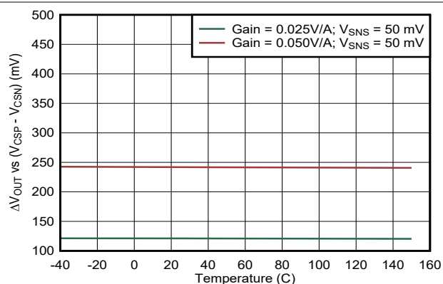
图 7-30. Cable Voltage Droop Compensation vs Temperature
