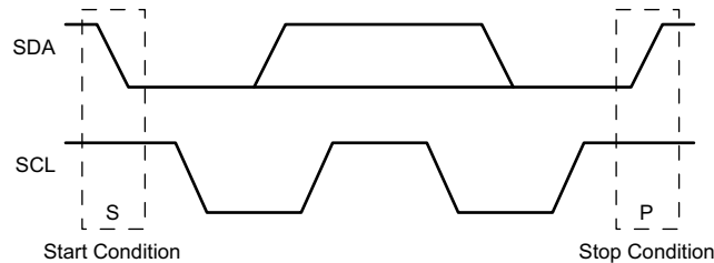
图 9-35. I²C Definition of Start and Stop Conditions
