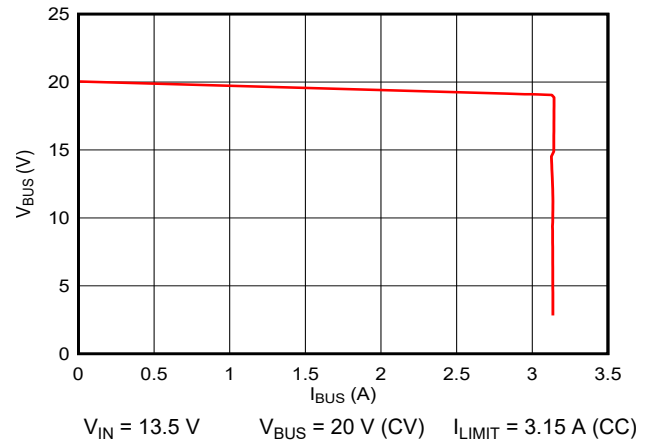
图 7-32. Constant Voltage to Constant Current Transition
