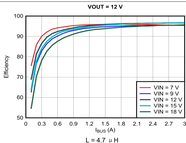
图 10-8. Efficiency vs Output Current ( I_{OUT} ), V_{OUT} = 12\text{ V}
