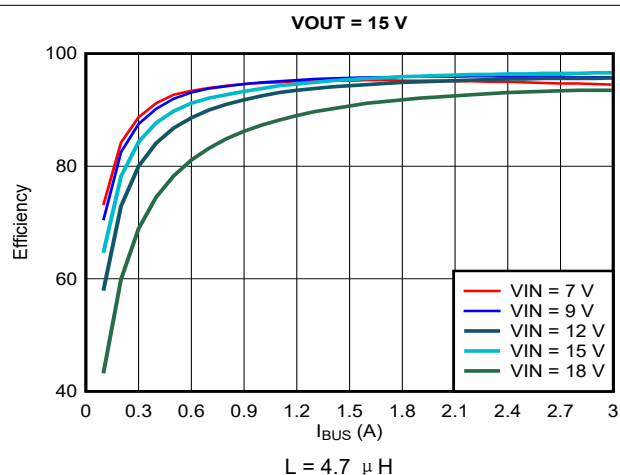
图 10-9. Efficiency vs Output Current ( I_{OUT} ), V_{OUT} = 15\text{ V}
