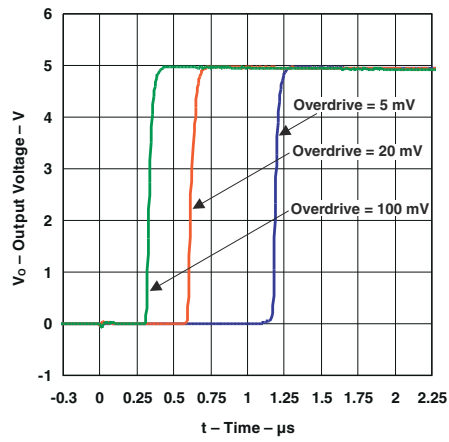
图 7-37. Response Time for Various Overdrives Positive Transition
