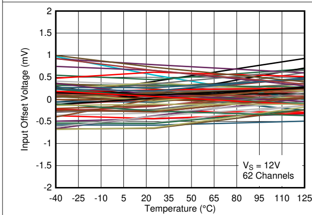
图 7-9. Input Offset Voltage vs. Temperature at 12V
