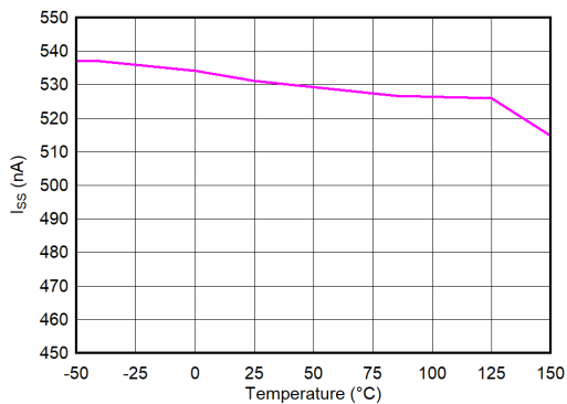
图 6-38. Soft-Start Charging Current (I SS ) vs Temperature (T J )
