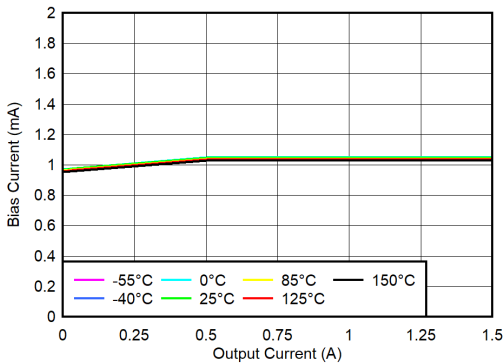
图 6-36. BIAS Pin Current vs Output Current and Temperature (T J )
