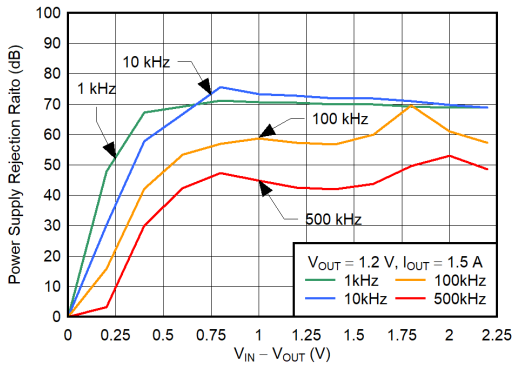
图 6-34. V IN PSRR vs (V IN - V OUT )
